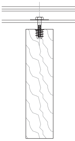
Strut Channel—Solid Wood
