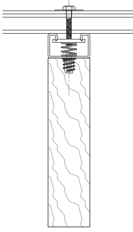
Strut to Strut—Solid Wood
