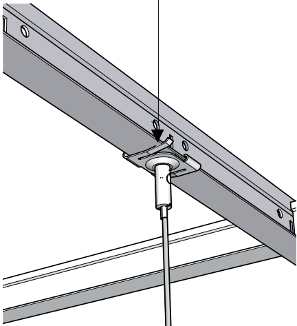
T-Bar attachment SKU:FF-TBA-ST-104
