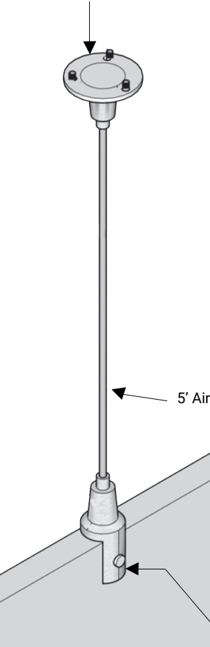
Ceiling & Floor Attachment SKU: FF-CA-ST-100 for upper ceiling and Concrete Slab with #8 - 2" Screw minimum by Installer
