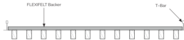
Ceiling Install—Lay-in
